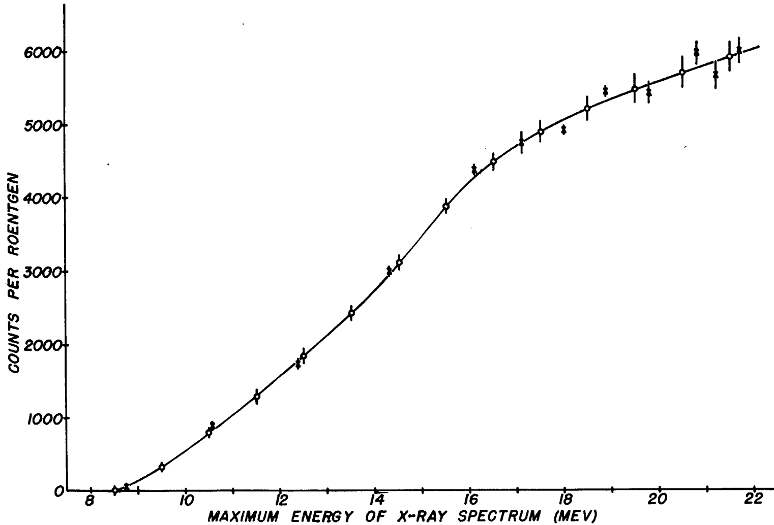
FIGURE 5 EXCITATION FUNCTION FOR U^{238}(\gamma, f)
