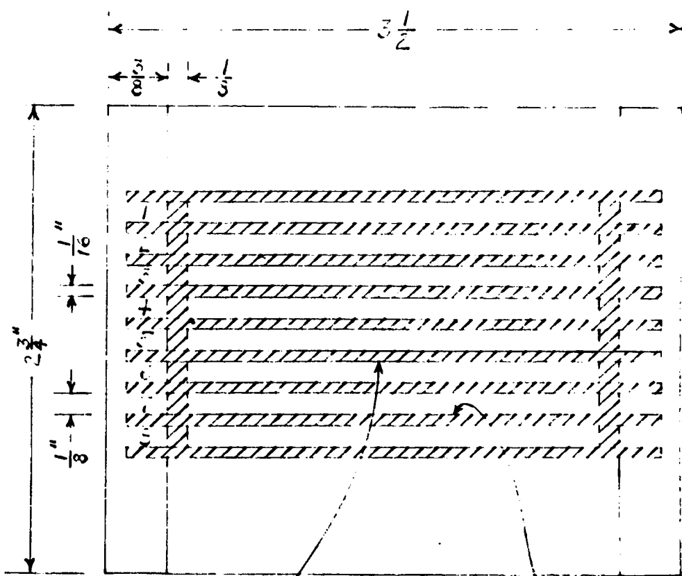
FIGURE 2 SAMPLE HOLDER
