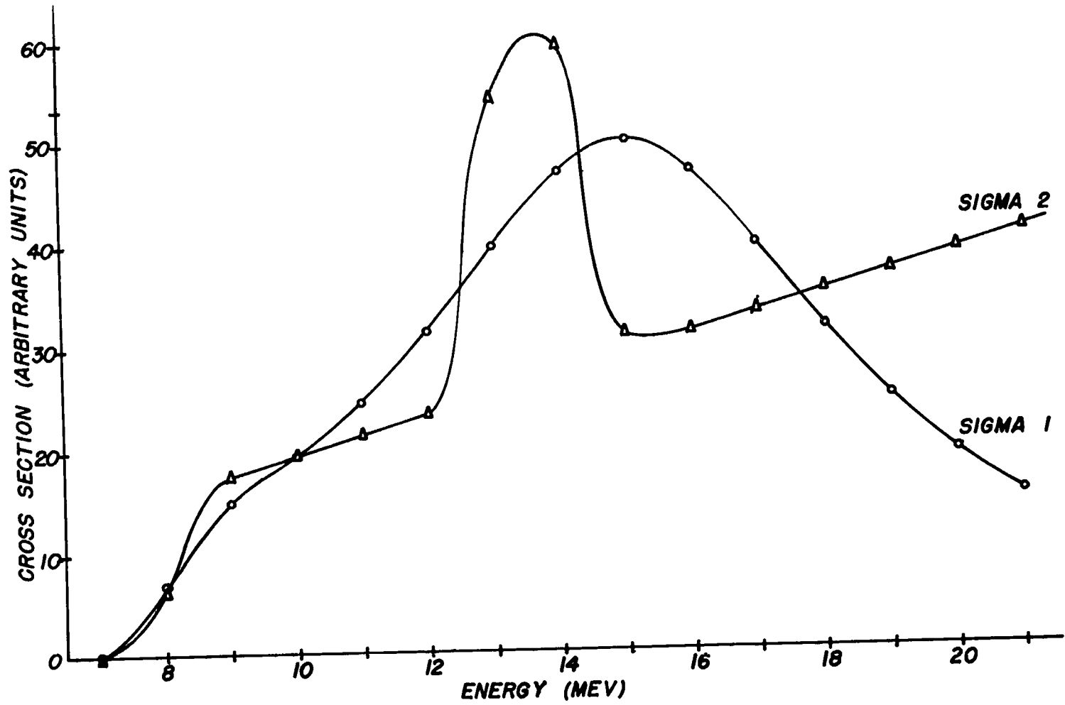
FIGURE 6 POSSIBLE (\gamma, f) CROSS SECTION SHAPES
